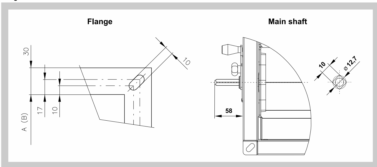
Fig. 6 Connection dimensions
