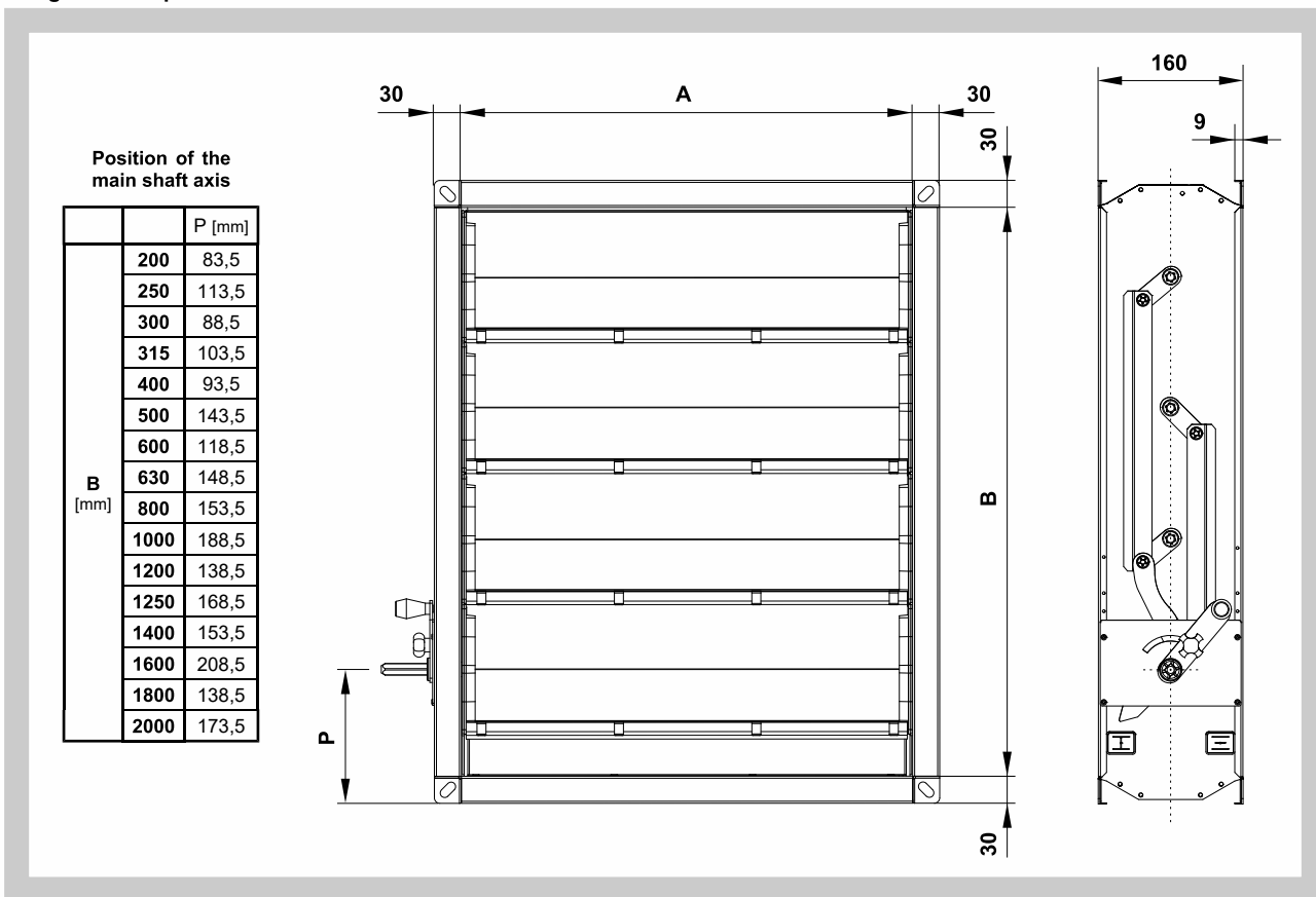
Fig. 5 Damper dimensions
