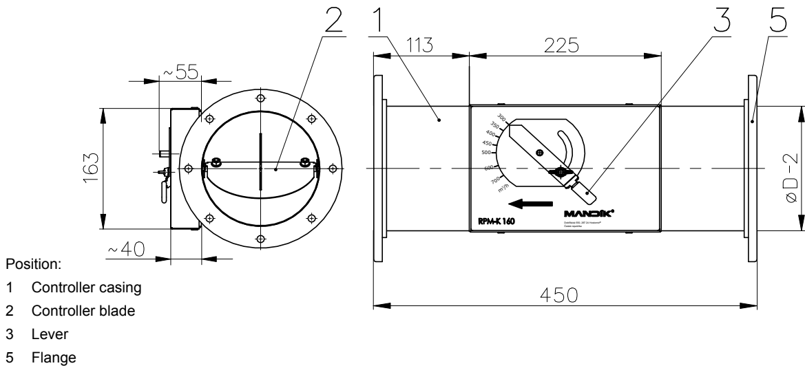
Fig. 4 Constant air volume regulator - with actuating mechanism
