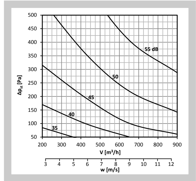
Diagram No. 14 Sound power level L_{WA} [dB(A)] radiated outside the pipeline DN250, without insulation
