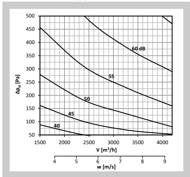
Diagram No. 39 Sound power level L_{WA} [dB(A)] radiated outside the pipeline 500x400, without insulation
