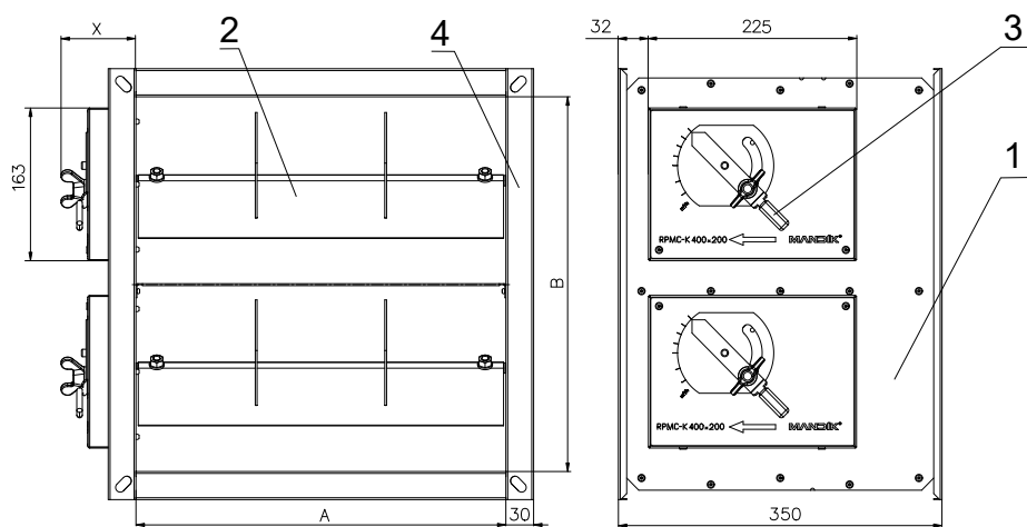
Fig. 6 Square constant air volume controller - B ≥ 400 mechanical control
