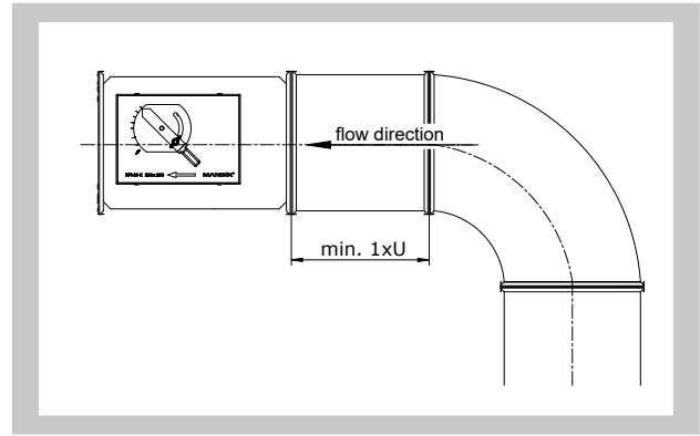
Fig. 8 Recommended distance from bend
