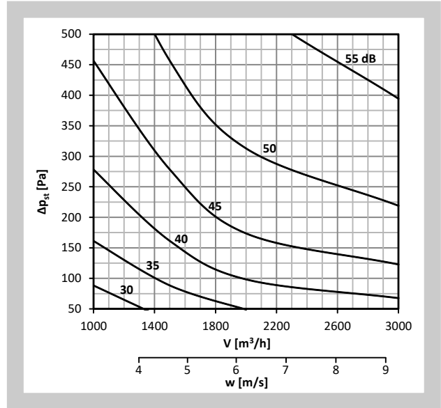
Diagram No. 56 Sound power level L_{WA} [dB(A)] radiated outside the pipeline 400x250, with insulation
