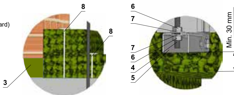
Insulation layers on the duct
