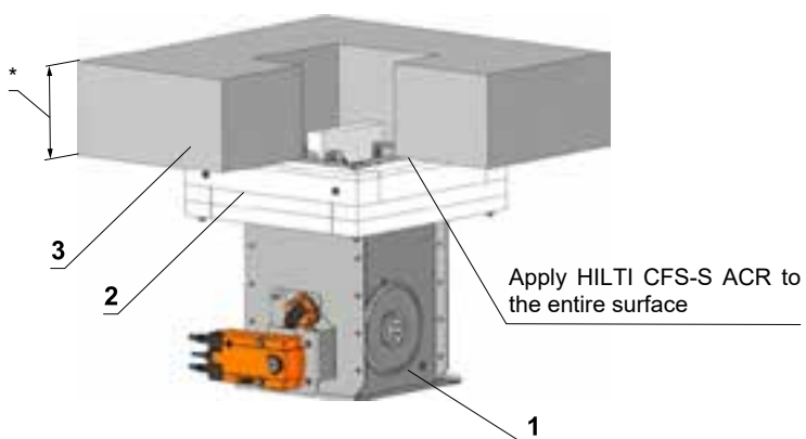
Installation frame E4
