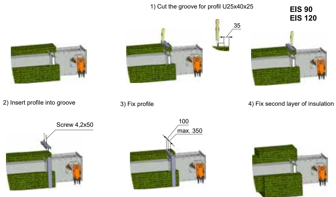
Fig. 81 Installation procedure
