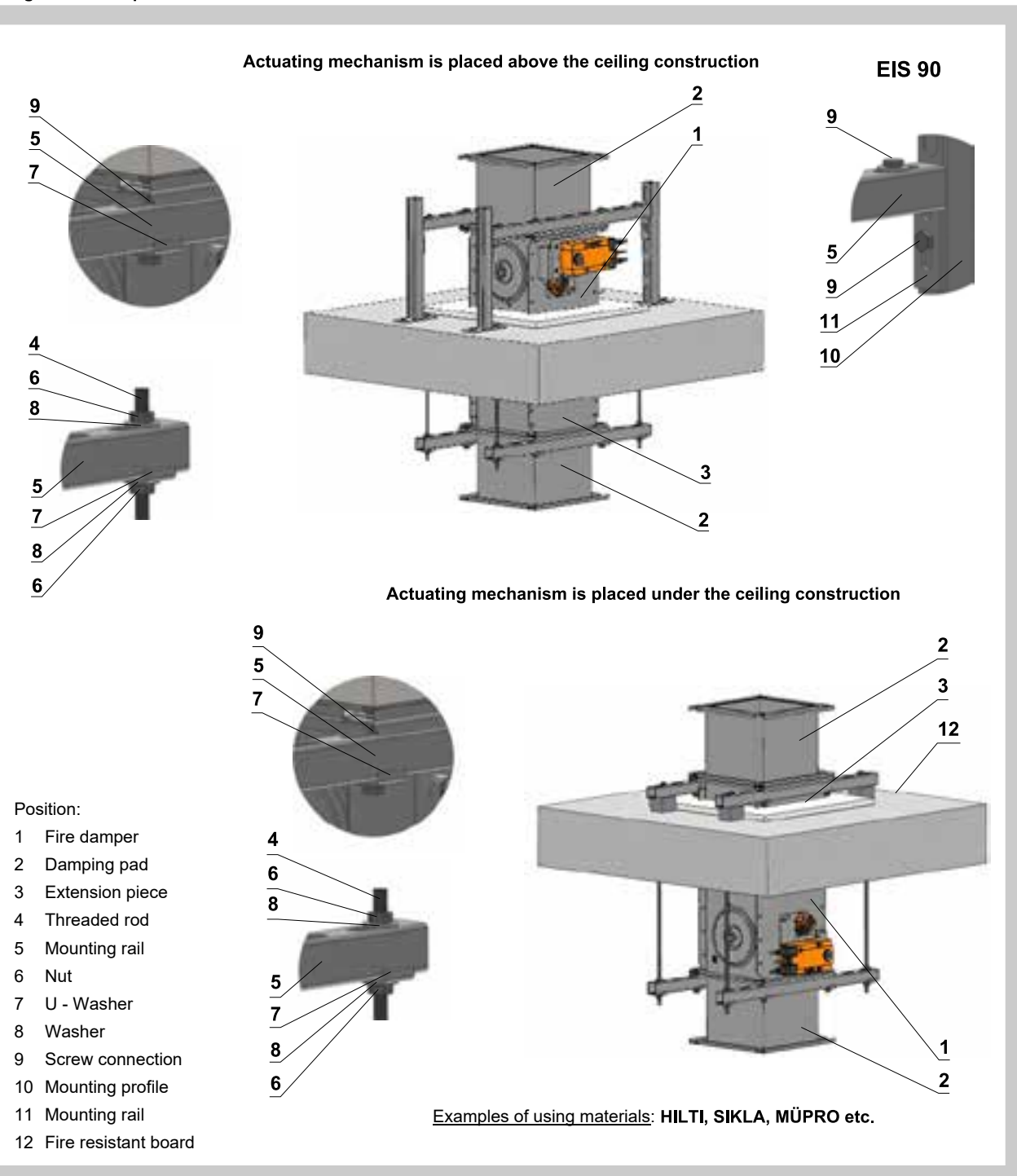
Fig. 86 Suspension - vertical duct
