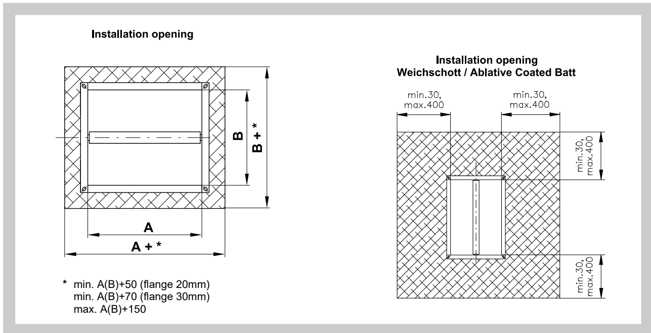
Fig. 33 Installation opening
