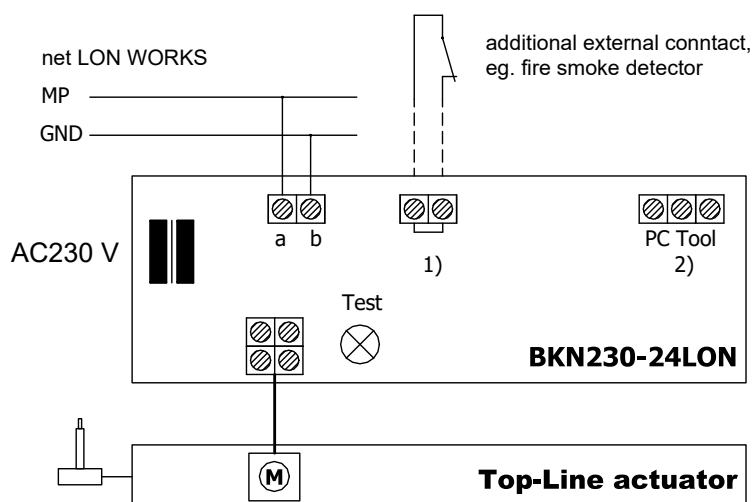
Fig. 23 Communication and supply device BKN 230-24LON
