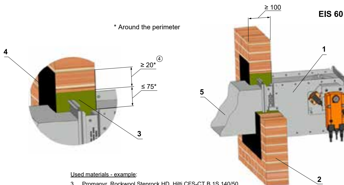
Fig. 35 Solid wall construction - stuffing box and fire protection mastic
