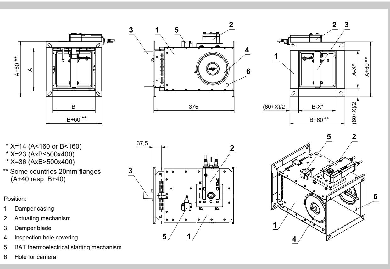
Fig. 27 Design with actuating mechanism
