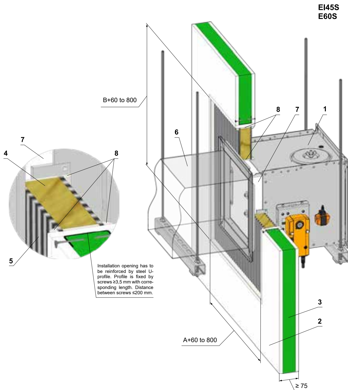
Fig. 54 Gypsum wall construction - Weichschott / Ablative Coated Batt
