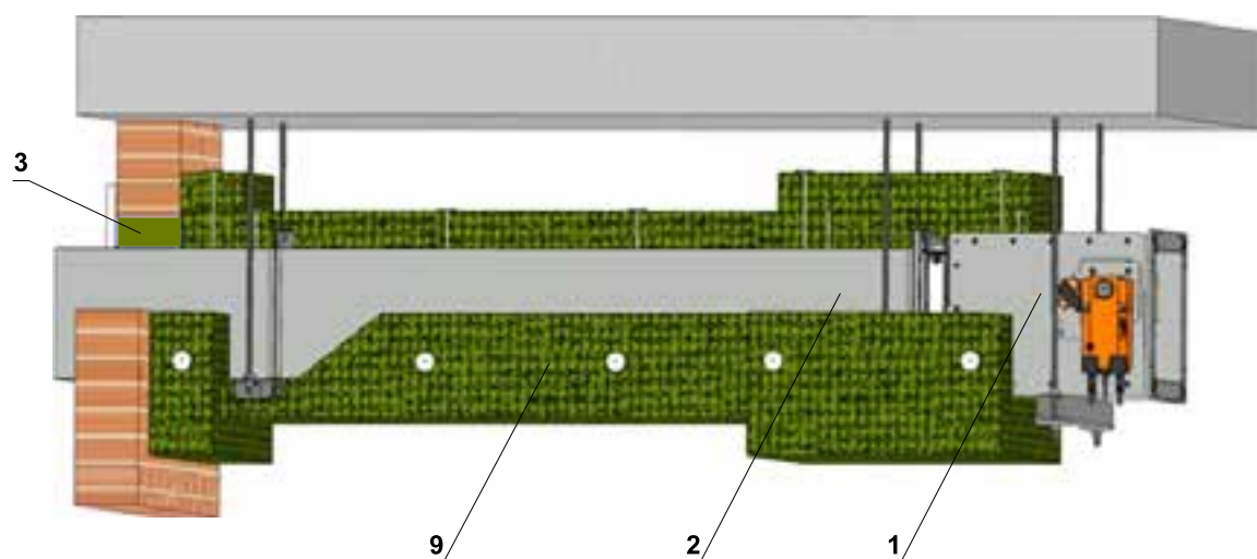
Insulation layers on the duct
