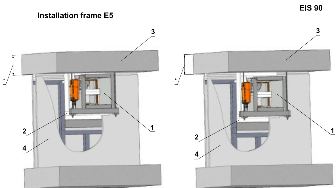
Fig. 57 Gypsum wall construction - flexible ceiling (with possibility to move/to sag) - installation frame E5
