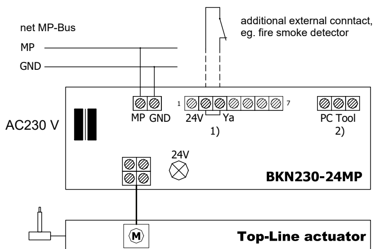
Fig. 22 Communication and supply device BKN 230-24MP
