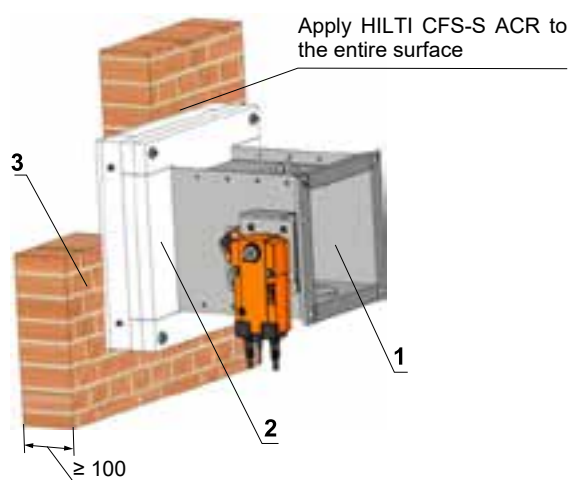
Installation frame E4
