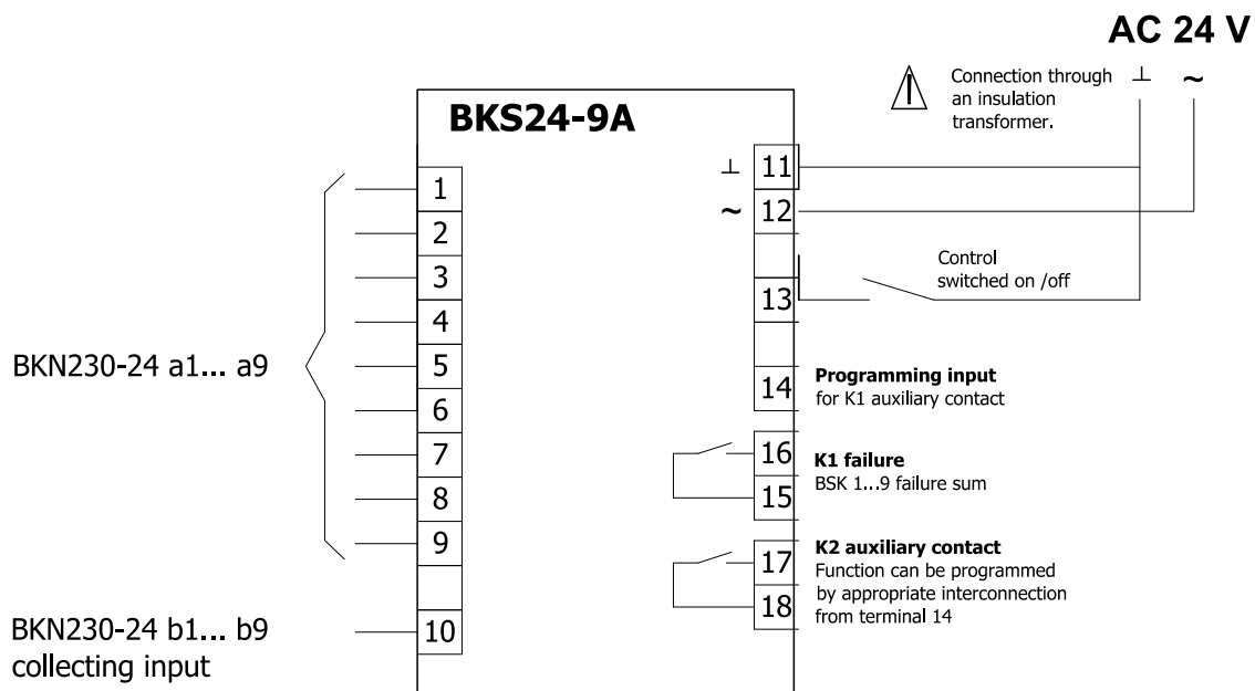
Fig. 25 Communication and control device BKS 24-9A
